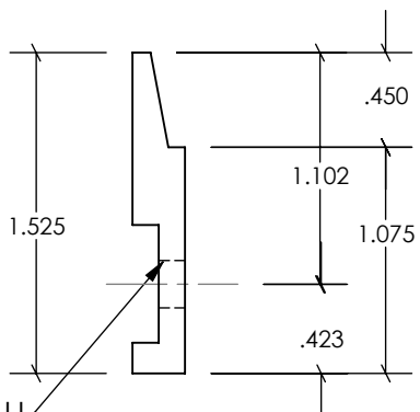
WALL CLEAT
